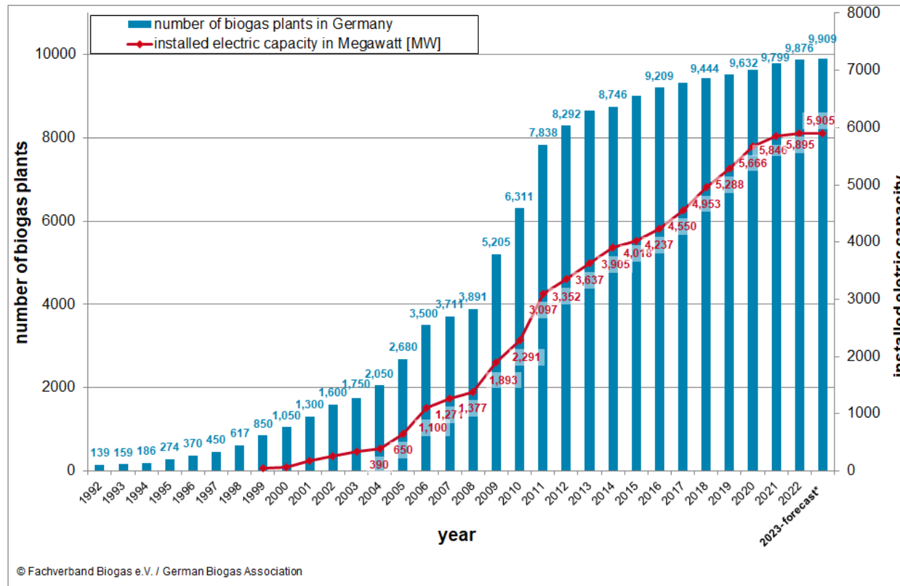
Development of the number of biogas plants and the total installed electric capacity in megawatt [MW] in Germany (as of 08/2023)
